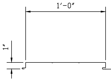
"HL-12" PANEL
